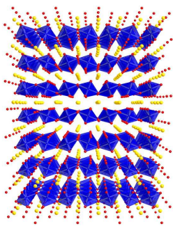
Structure post-perovskite
